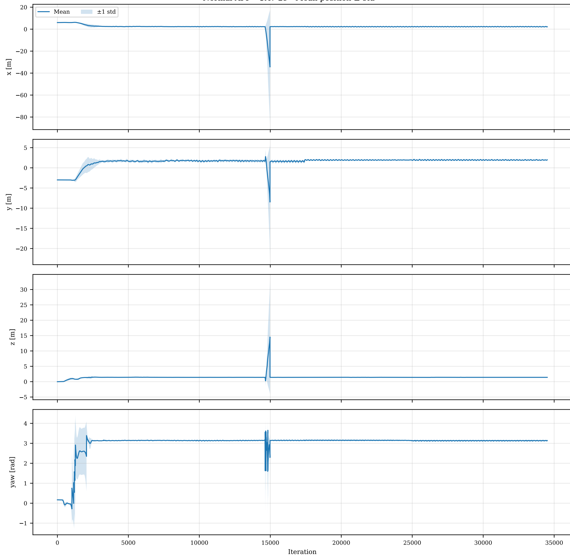
Normal APF - UAV 29 - Mean position \pm std
